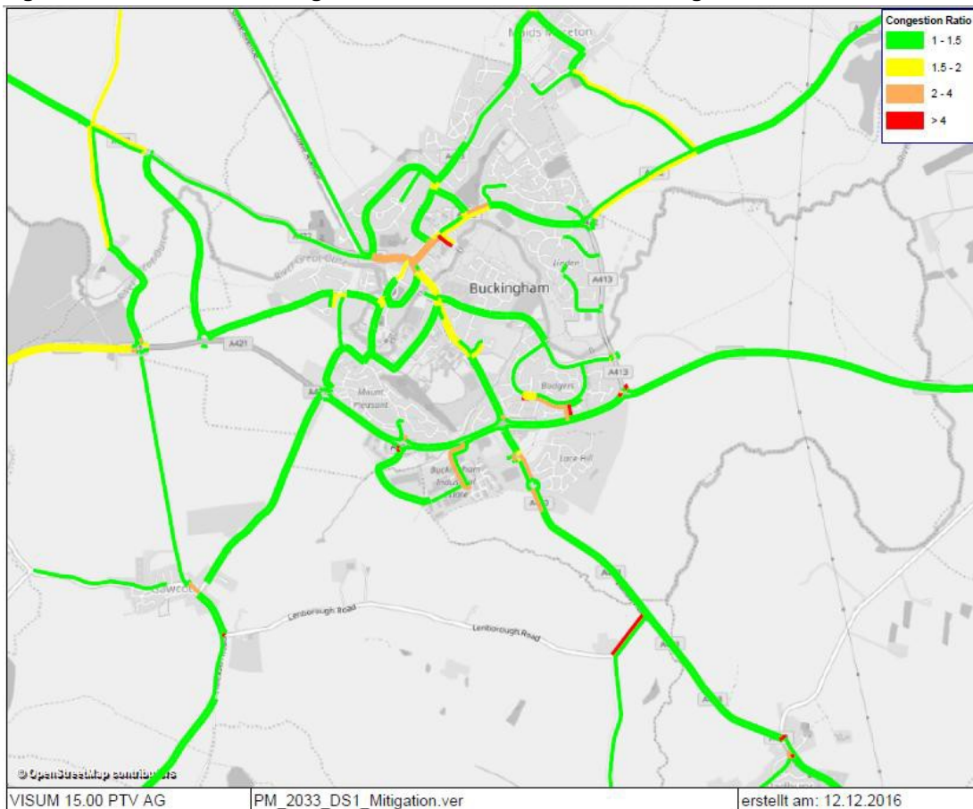
Figure 4.13: PM Peak with mitigation – Performance Plots in Buckingham, 2033 73
