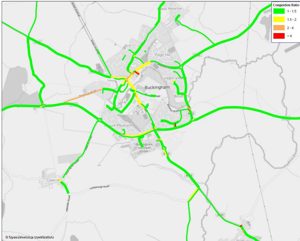
Figure 2.22: PM Peak Performance Plots in Buckingham, 2013 38
